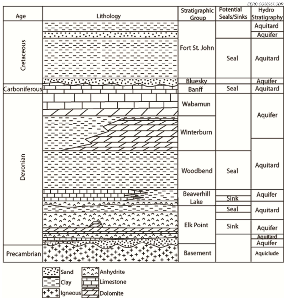
Figure 4. Stratigraphic and hydrostratigraphic delineation and nomenclature as well as general lithology for the northern part of the Alberta Basin, including northeastern British Columbia (modified from British Columbia Ministry of Energy, Mines, and Petroleum Resources, 2007).
